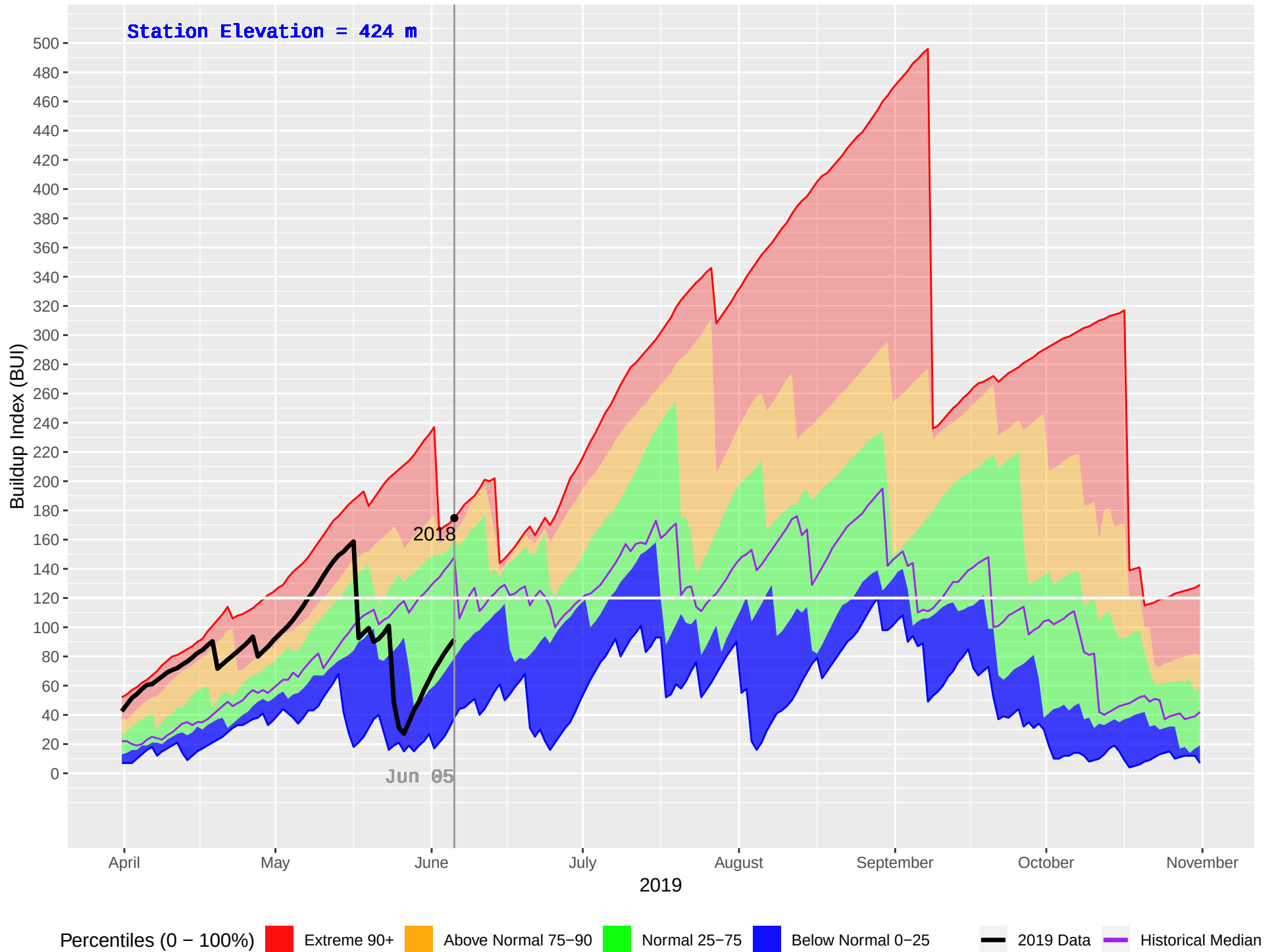
SPLINTLUM (1055) : Historical (2009–2018), Current (2019) Daily Buildup Index (BUI)
