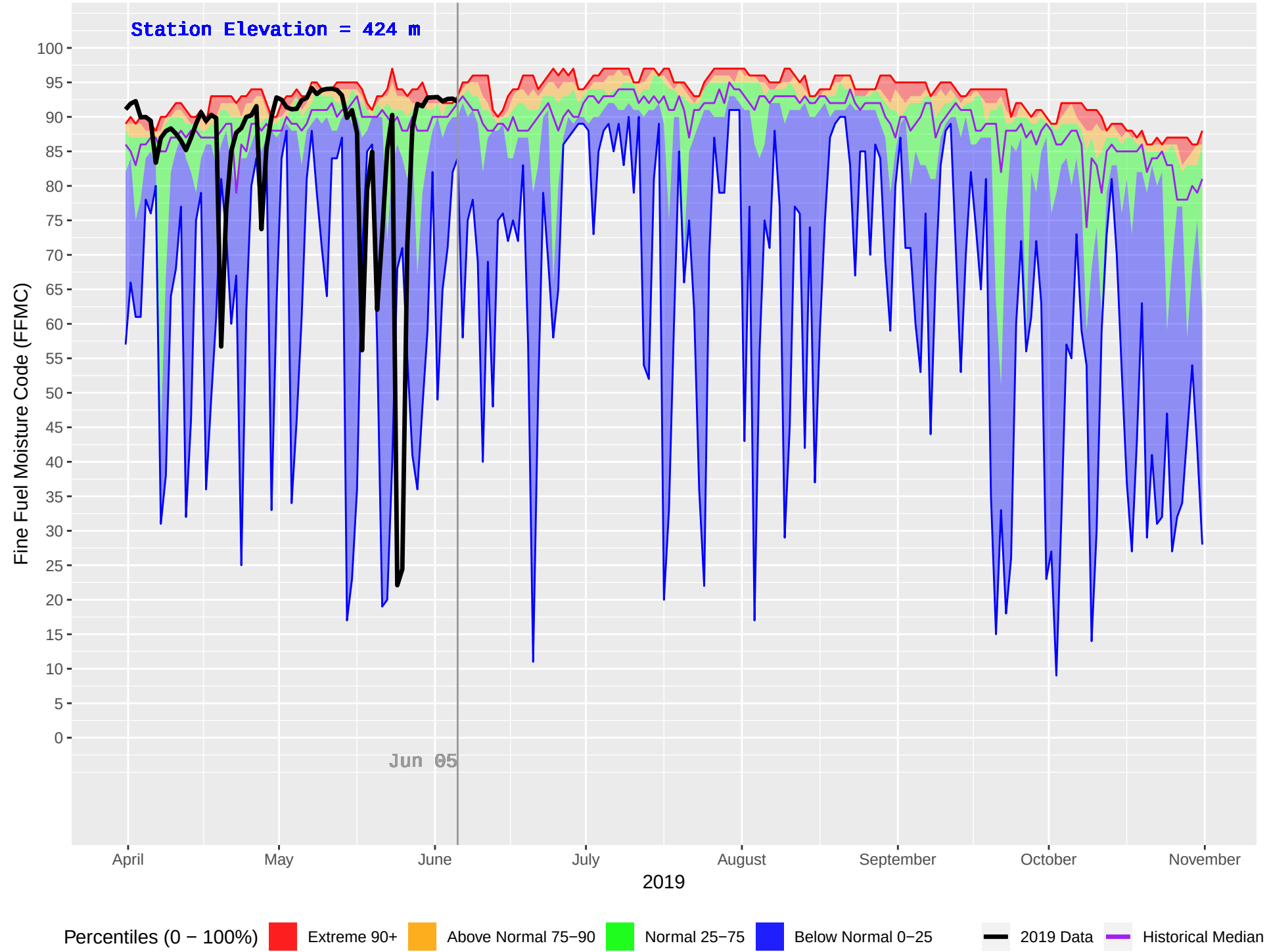
SPLINTLUM (1055) : Historical (2009–2018) and Current (2019) Daily Fine Fuel Moisture Code (FFMC)
