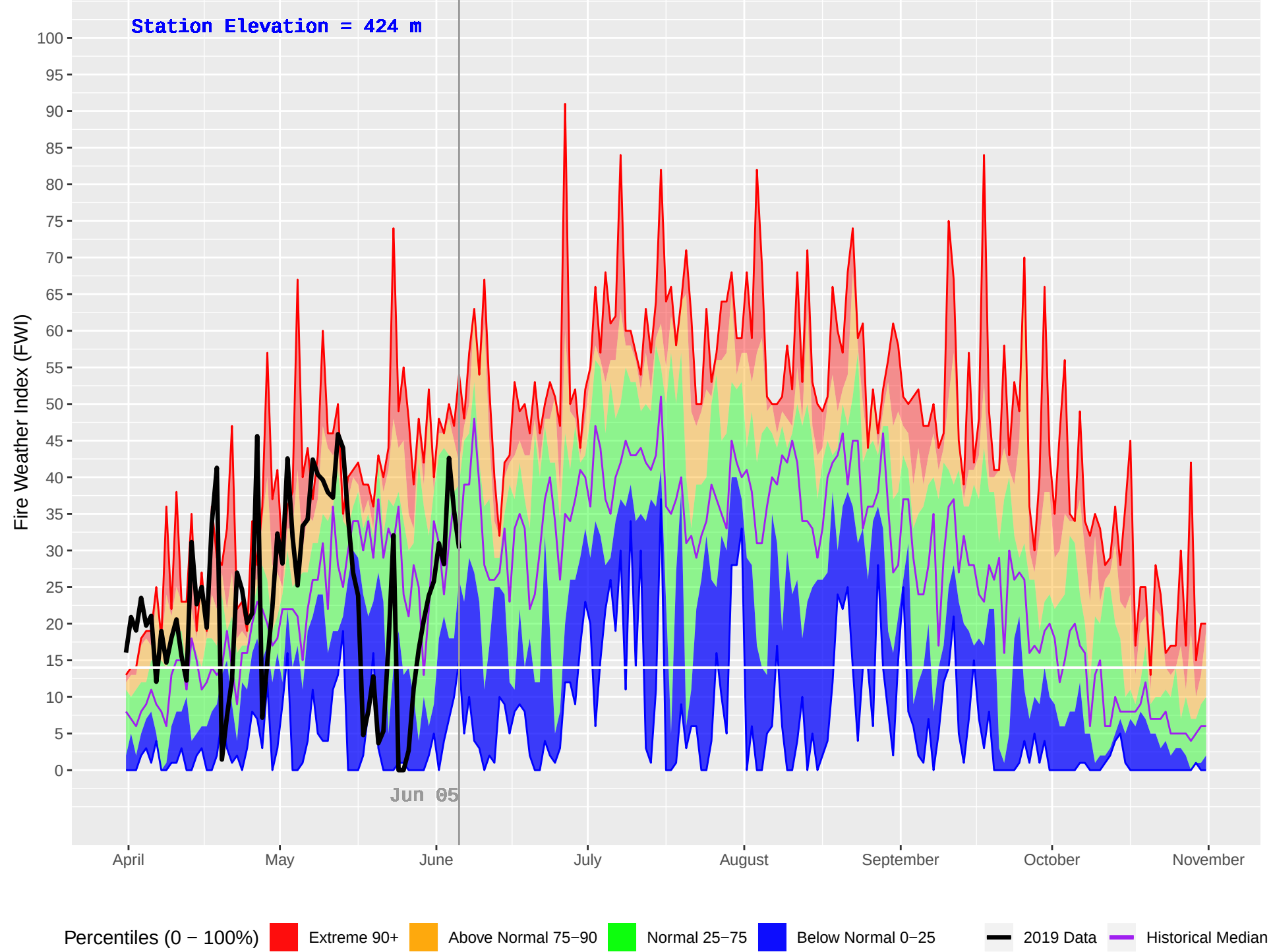
SPLINTLUM (1055) : Historical (2009–2018) and Current (2019) Daily Fire Weather Index (FWI)
