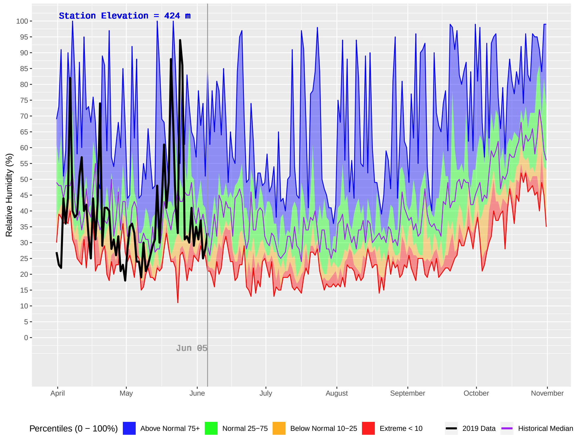
SPLINTLUM (1055) : Historical (2009–2018) and Current (2019) Daily Relative Humidity
