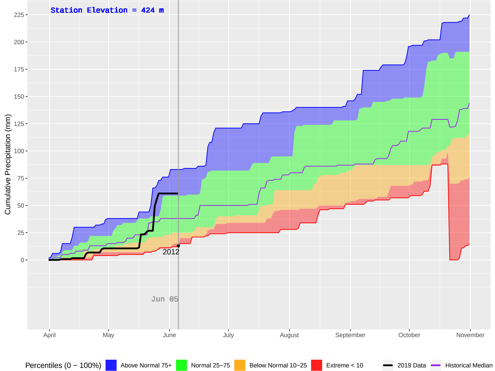
SPLINTLUM (1055) : Historical (2009–2018), Current (2019) Daily Cumulative Precipitation
