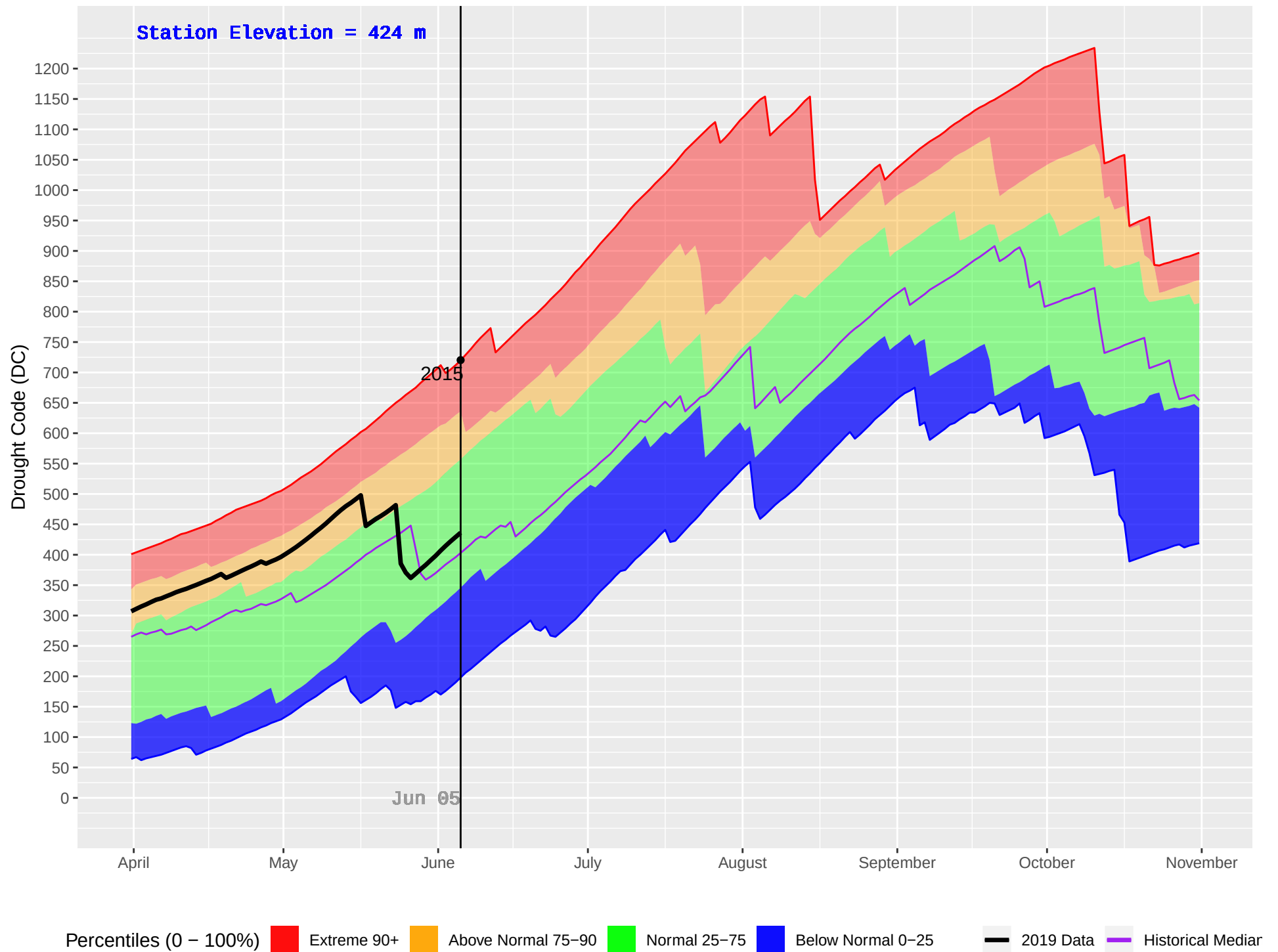
SPLINTLUM (1055) : Historical (2009–2018) and Current (2019) Daily Drought Code (DC)
