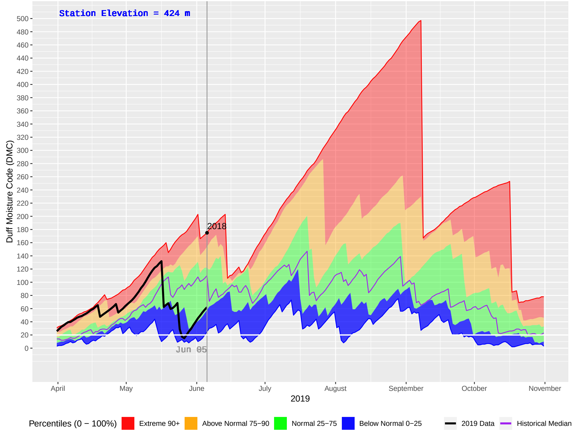
SPLINTLUM (1055) : Historical (2009–2018), Current (2019) Daily Duff Moisture Code (DMC)
