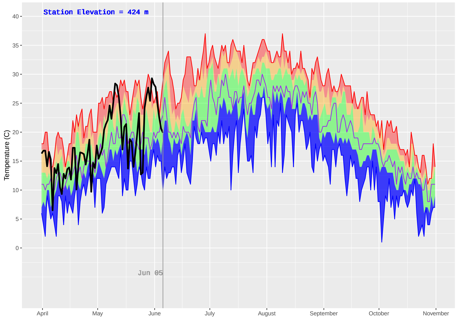
SPLINTLUM (1055) : Historical (2009–2018) and Current (2019) Daily Temperature
